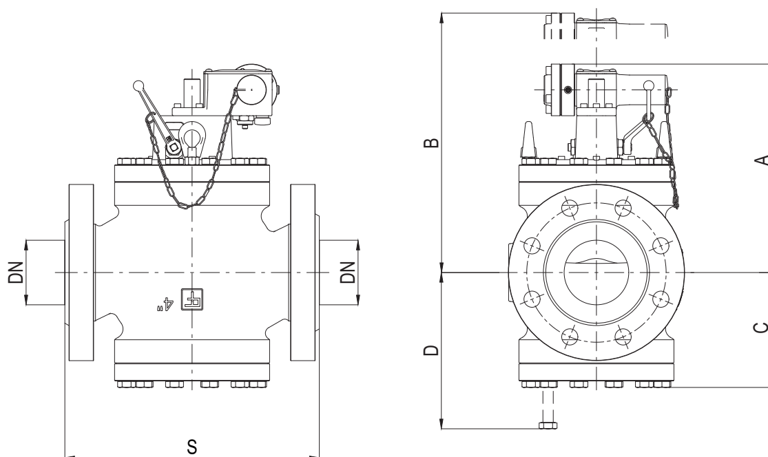
Figure 6 SBC 782 dimensions
