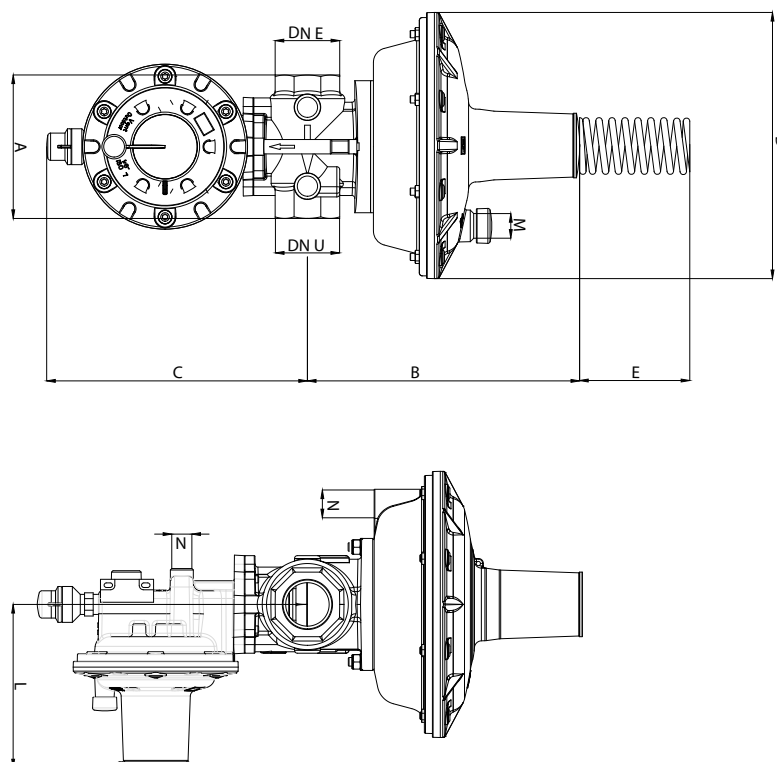
Figure 9 Dival 507-512 + LA dimensions
