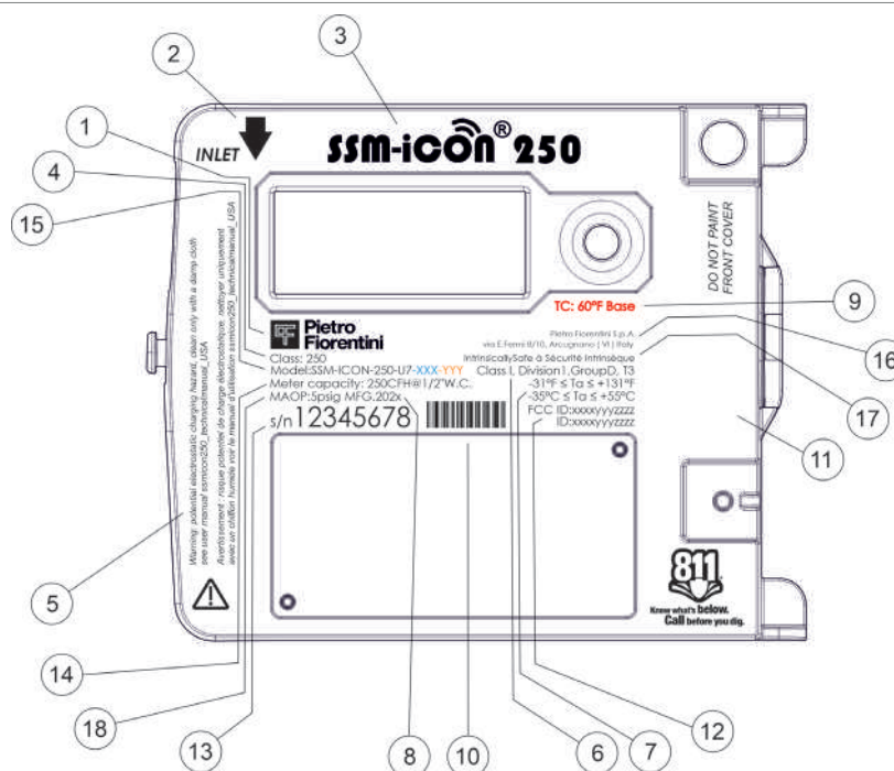
Fig. 2.1. Description of identification plates
