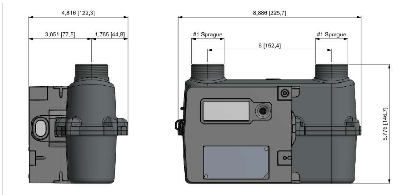
Fig. 6.6. SSM-ICON 250 Standard Dimensions
