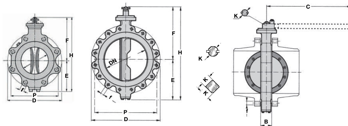
Figure 4 BF 31 dimensions
