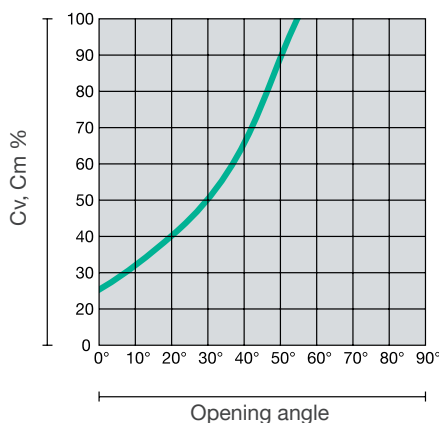
Figure 3 BF 31 CM, Cvm curves
