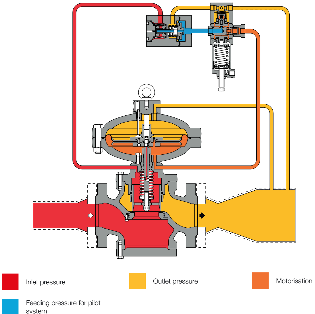
Figure 2 Reflux 819
