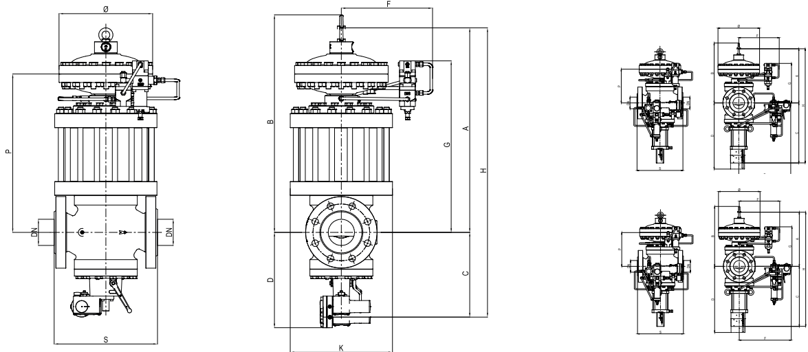
Figure 14 Reflux 819 + DB/819 + SB/82 or HB/97 dimensions
