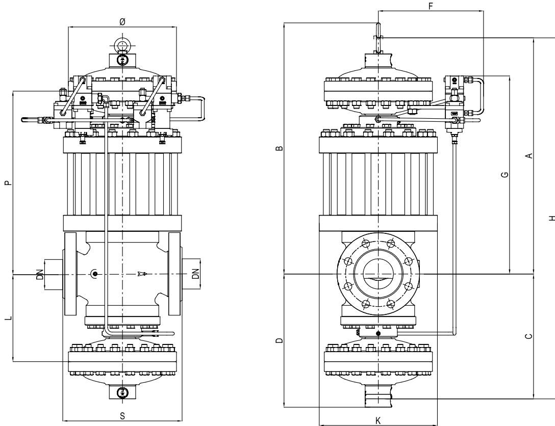
Figure 15 Reflux 819 + DB/819 + PM/819 dimensions
