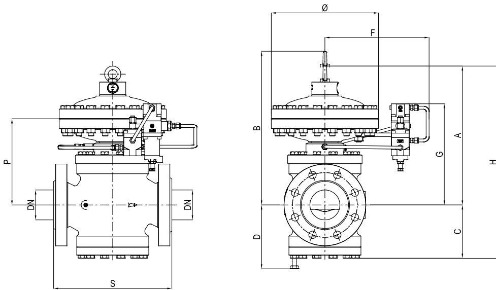
Figure 10 Reflux 819 dimensions
