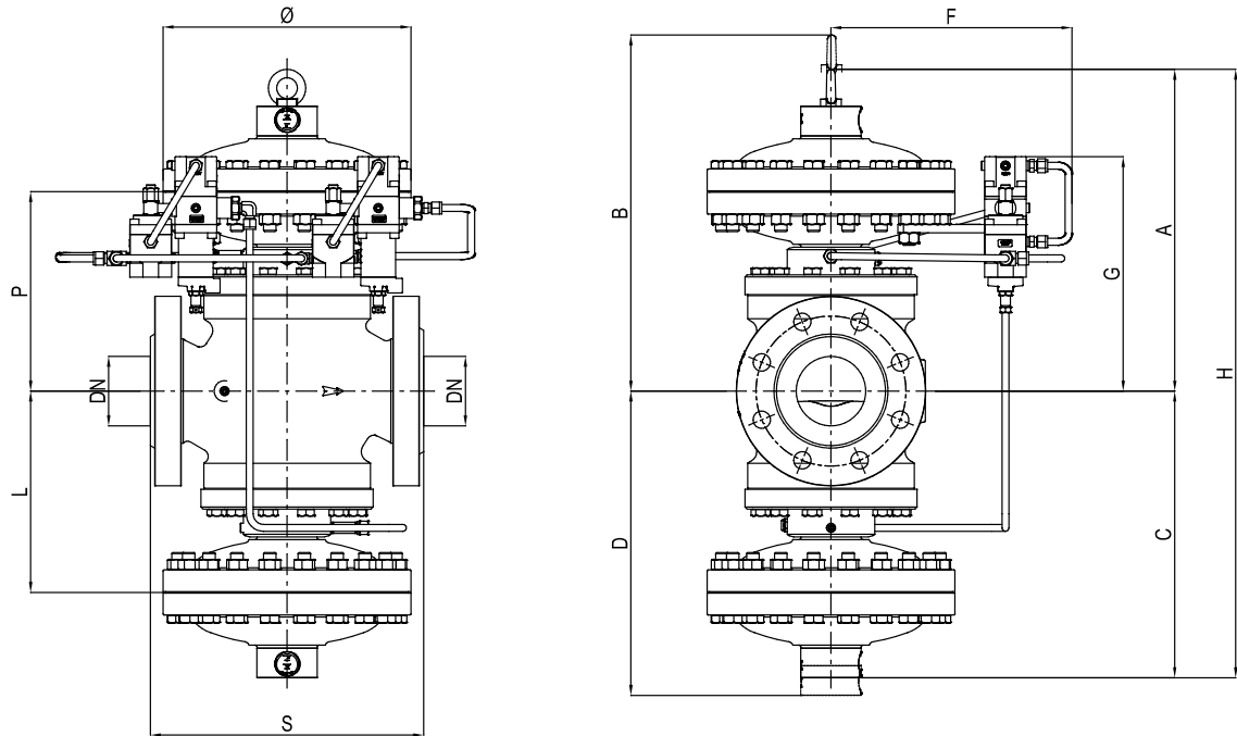
Figure 12 Reflux 819 + PM/819 dimensions
