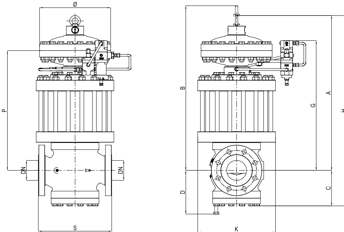
Figure 13 Reflux 819 + DB/819 dimensions
