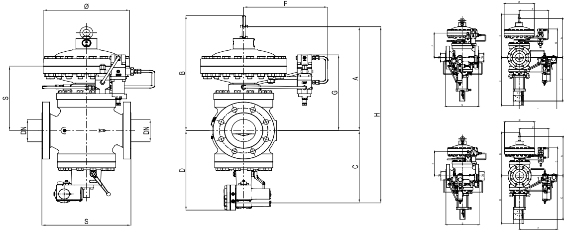
Figure 11 Reflux 819 + SB/82 or HB/97 dimensions
